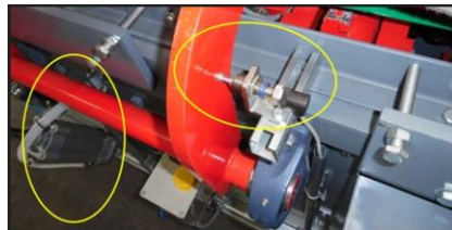
Operation of the cylinder position sensor
