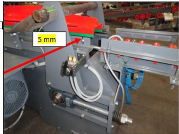
Operation of the cylinder position sensor
